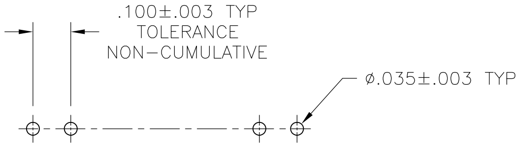
RECOMMENDED HOLE LAYOUT
