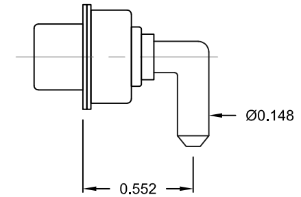
40 AMP POWER CONTACT
