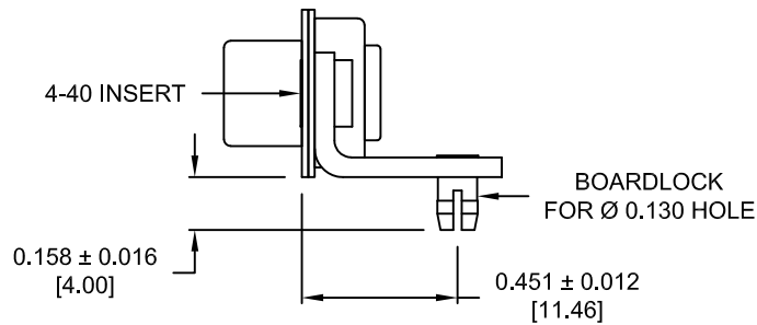
MOUNTING HARDWARE
