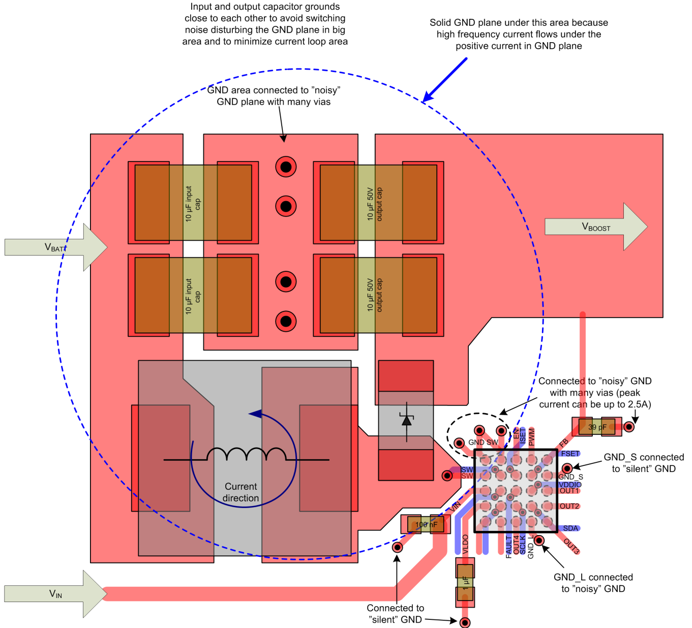
Figure 33. LP8552 Layout
