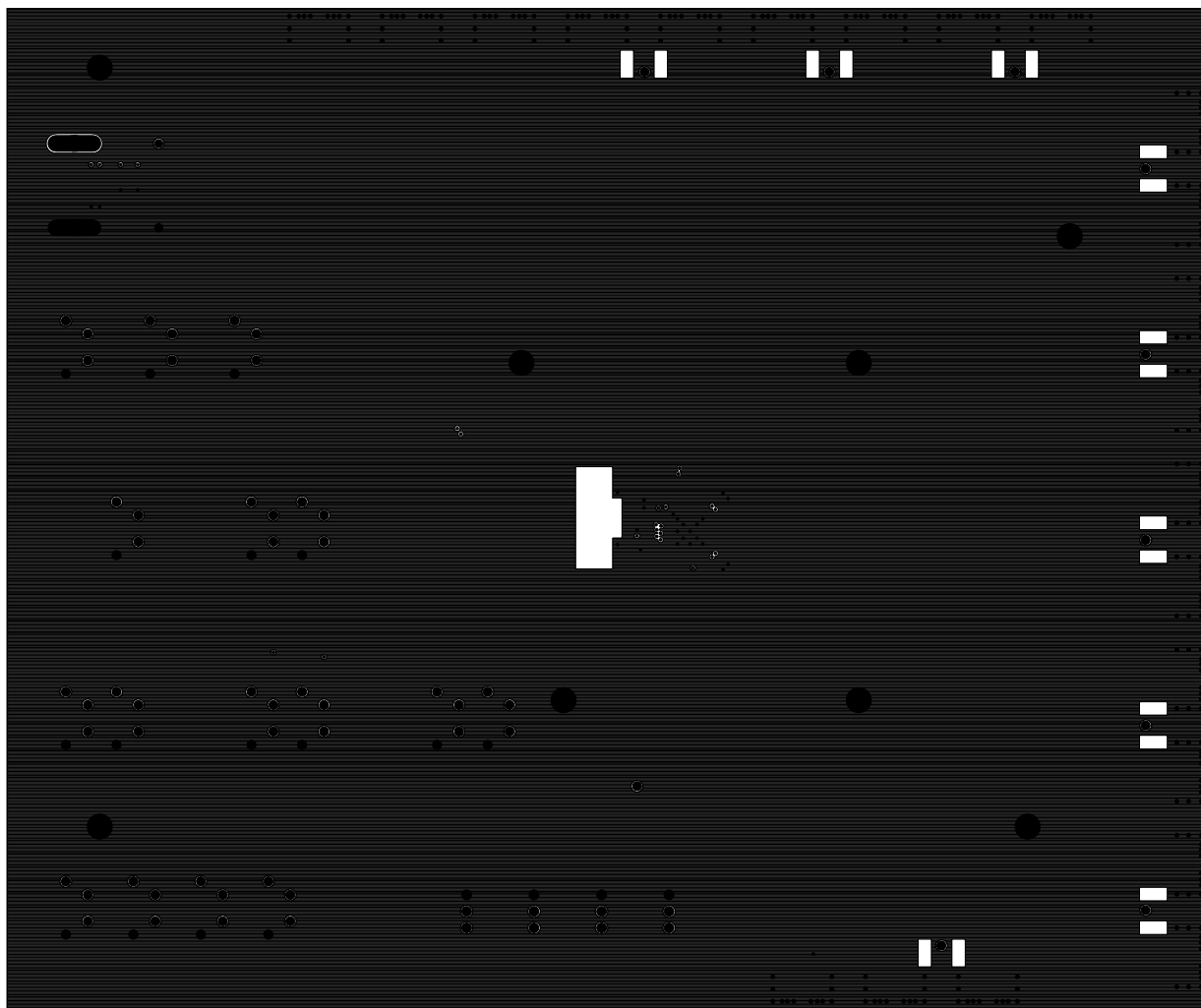
Figure 5. MAX3637 EV Kit PCB Layout—Ground Plane
