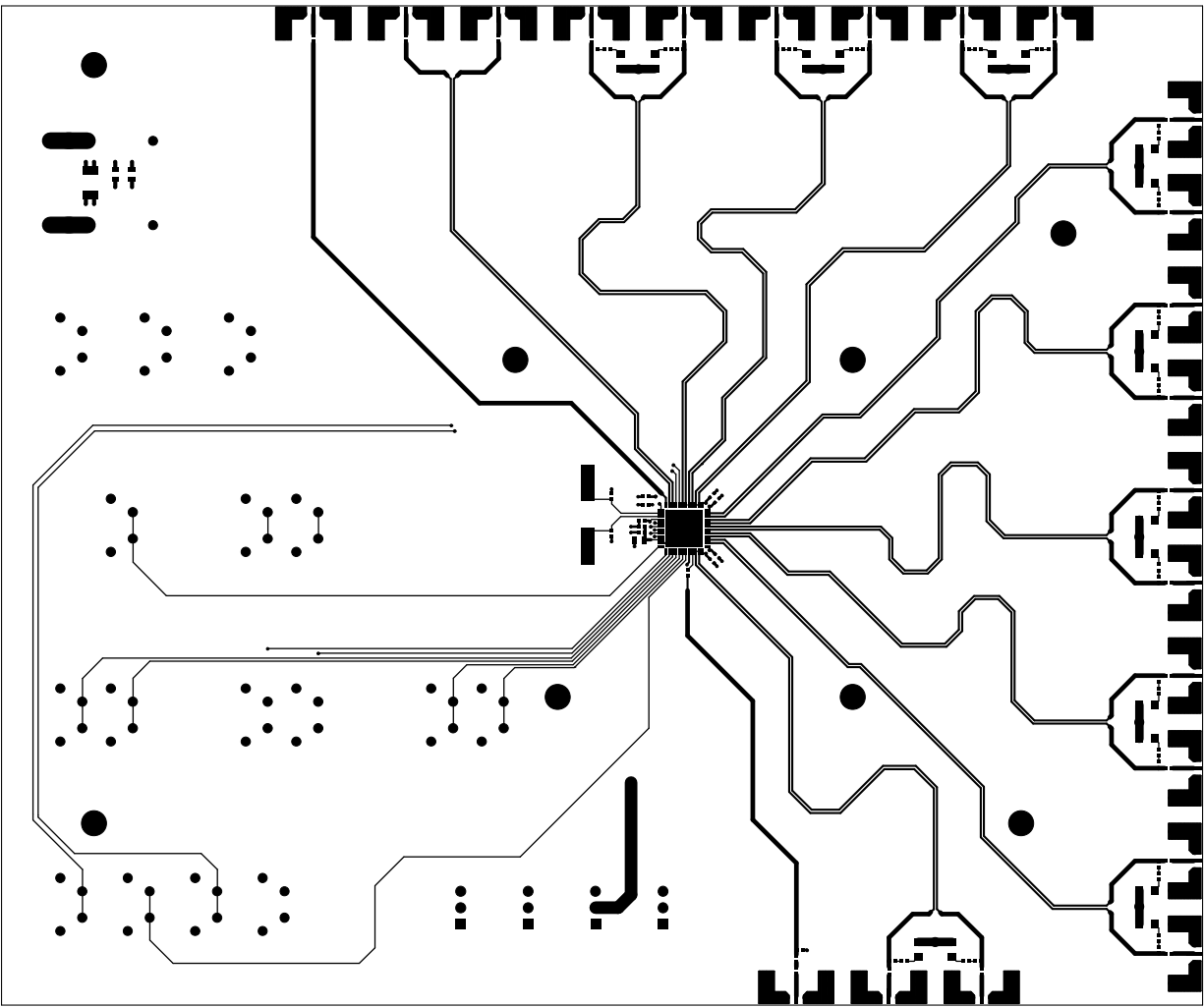
Figure 4. MAX3637 EV Kit PCB Layout—Component Side
