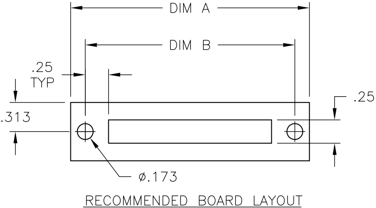
RECOMMENDED BOARD LAYOUT
