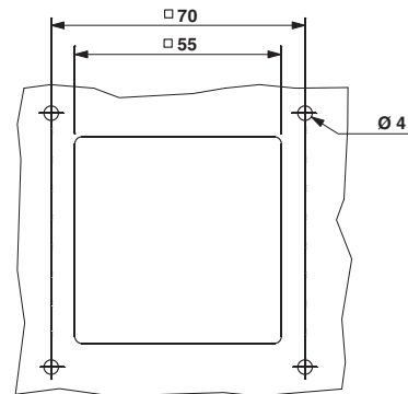
Panel cutout: DC-B 6-HB-M
