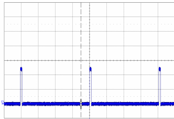
Figure 14. Load current (5A/div., 50 ms/div.) into a 10 m \Omega short circuit during restart, at V_{in} = 48 V.
