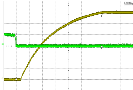
Figure 7. Turn-on transient at full rated load current (resistive) plus 5,000 \mu\text{F} at V_{in}=48\text{V} , triggered via ON/OFF pin. Top trace: ON/OFF signal (5V/div.). Bottom trace: Output voltage (2V/div.). Time scale: 2ms/div.
