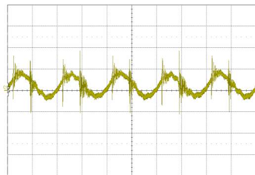
Figure 9. Output voltage ripple (20 mV/div.) at full rated load current into a resistive load with C_o = 10\mu\text{F} tantalum + 1\mu\text{F} ceramic and V_{in} = 48\text{V} . Time scale: 1 \mu\text{s} /div.
