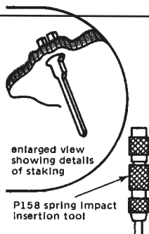
FIG. 1 Backup Method Solder Terminals Only. Also See FIGS. 6 & 7.
