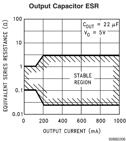
FIGURE 1. ESR Limits
