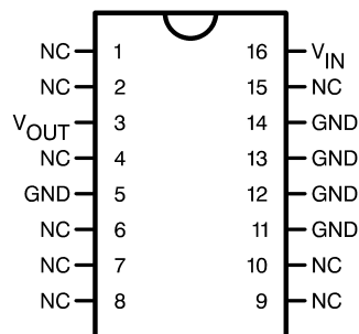
16-Lead Dual-in-Line Package (J)
