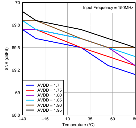
Figure 119. SNR vs Temperature and AVDD Supply
