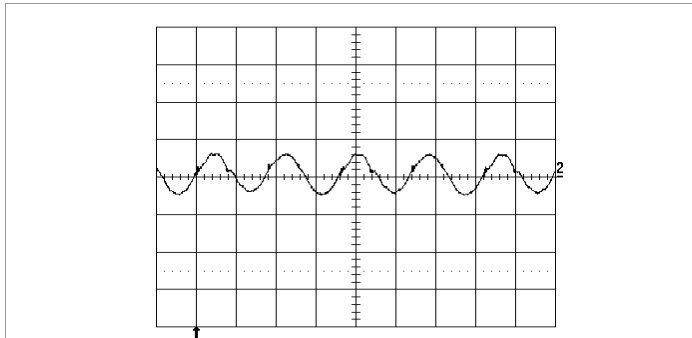
Output voltage ripple at: T_{P1}, T_{P3} = +25^{\circ}\text{C}, V_1 = 53\text{ V}, I_O = 35\text{ A} resistive load. Trace: output voltage (50 mV/div.). Time scale: (2 \mu\text{s} /div.).
