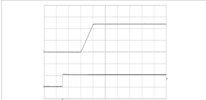
Start-up enabled by connecting V_1 at: T_{P1}, T_{P3} = +25^{\circ}\text{C}, V_1 = 53\text{ V}, I_O = 35\text{ A} resistive load. Top trace: output voltage (5 V/div.). Bottom trace: input voltage (50 V/div.). Time scale: (10 ms/div.).
