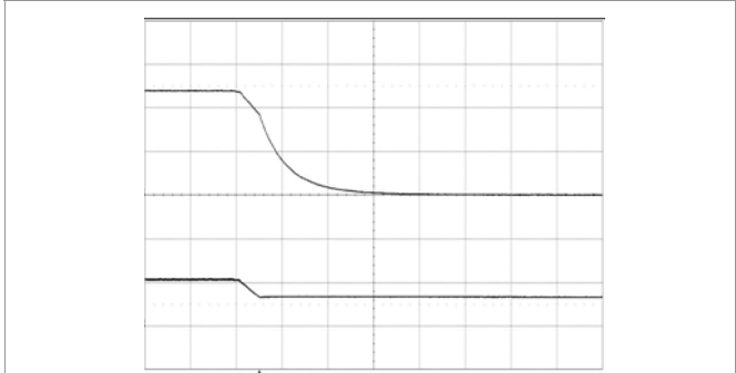
Shut-down enabled by disconnecting V_1 at: T_{P1}, T_{P3} = +25^{\circ}\text{C}, V_1 = 53\text{ V}, I_O = 35\text{ A} resistive load. Top trace: output voltage (5 V/div.). Bottom trace: input voltage (50 V/div.). Time scale: (2 ms/div.).
