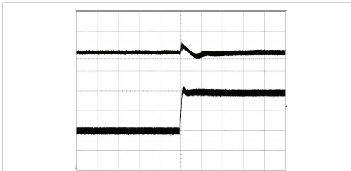
Output voltage response to input voltage transient at: T_{P1}, T_{P3} = +25^{\circ}\text{C}, V_1 = 36-75\text{ V}, I_O = 17\text{ A} resistive load, C_O = 3.5\text{ mF} Top trace: output voltage (2 V/div.). Bottom trace: input voltage (20 V/div.). Time scale: (0.5 ms/div.).
