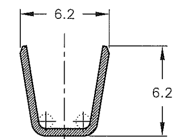
断面 "A"- "A" SECT "A"- "A"
