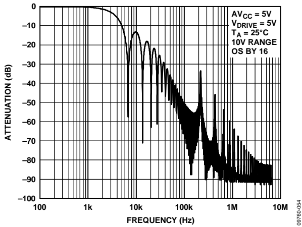
Figure 57. Digital Filter Response for OS × 16
