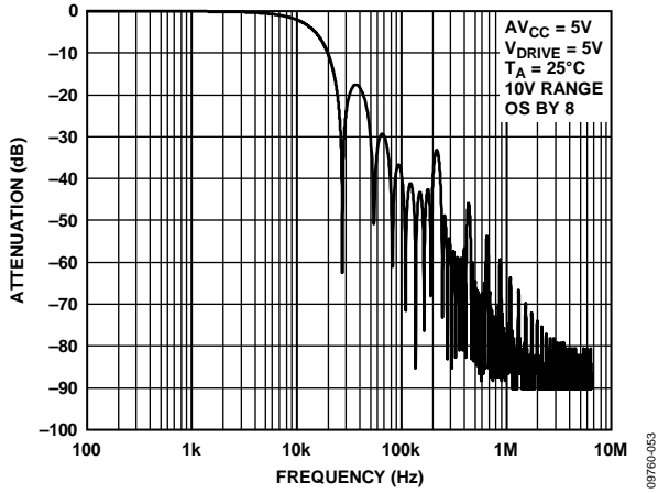
Figure 56. Digital Filter Response for OS × 8
