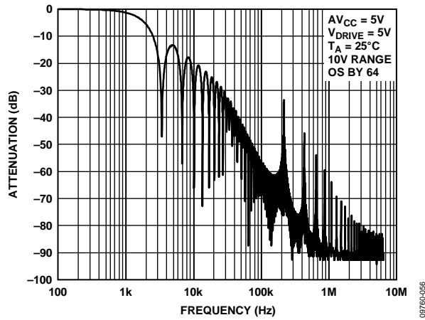
Figure 59. Digital Filter Response for OS × 64
