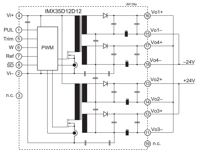
Fig. 7 Generating 24 V with an IMX35D12D12-9
