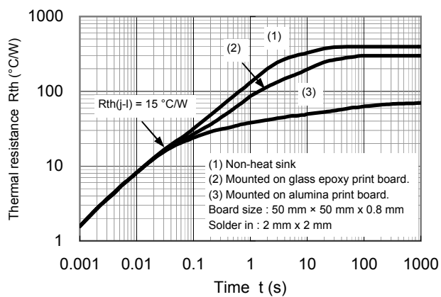
Rth - t
