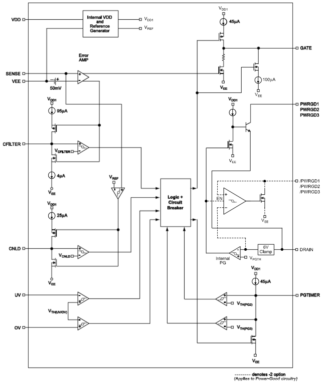
Block Diagram
