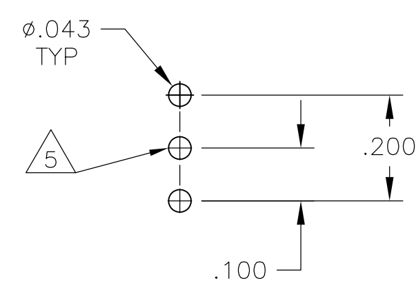
PCB HOLE LAYOUT
