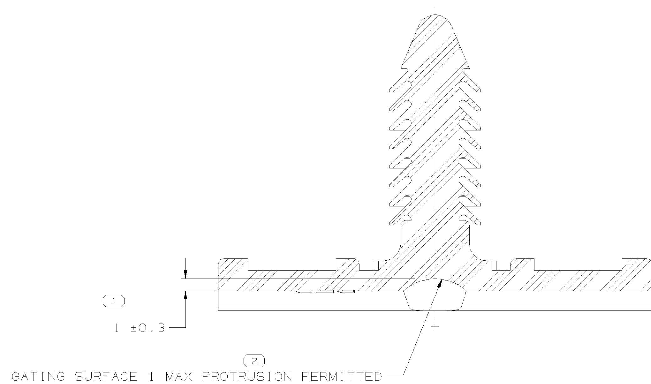
SECTION A-A OPTIONAL CONSTRUCTION
