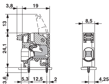
Dimensional drawing
