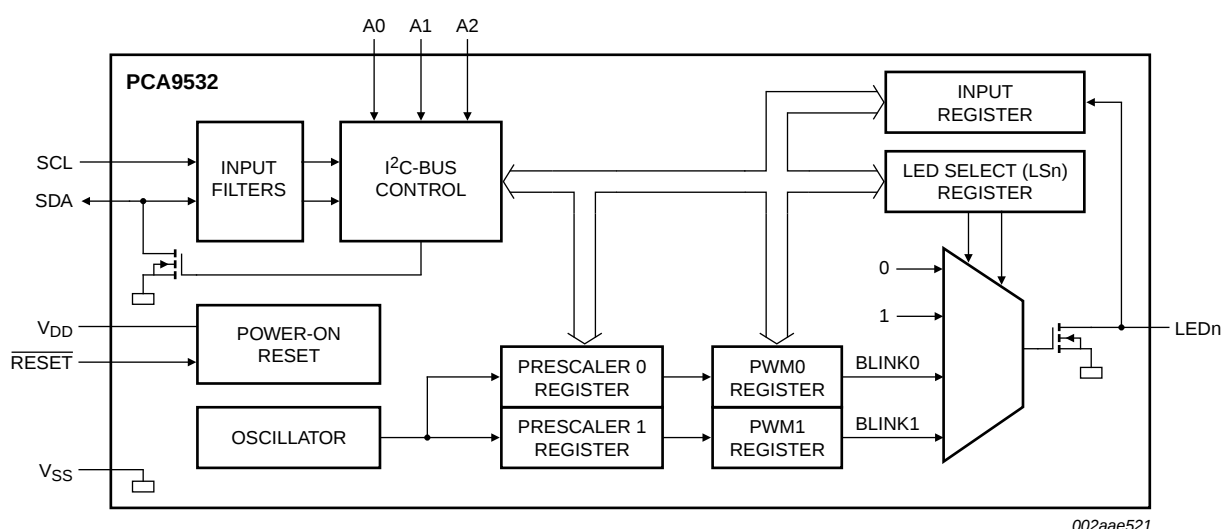
Fig 1. Block diagram of PCA9532
