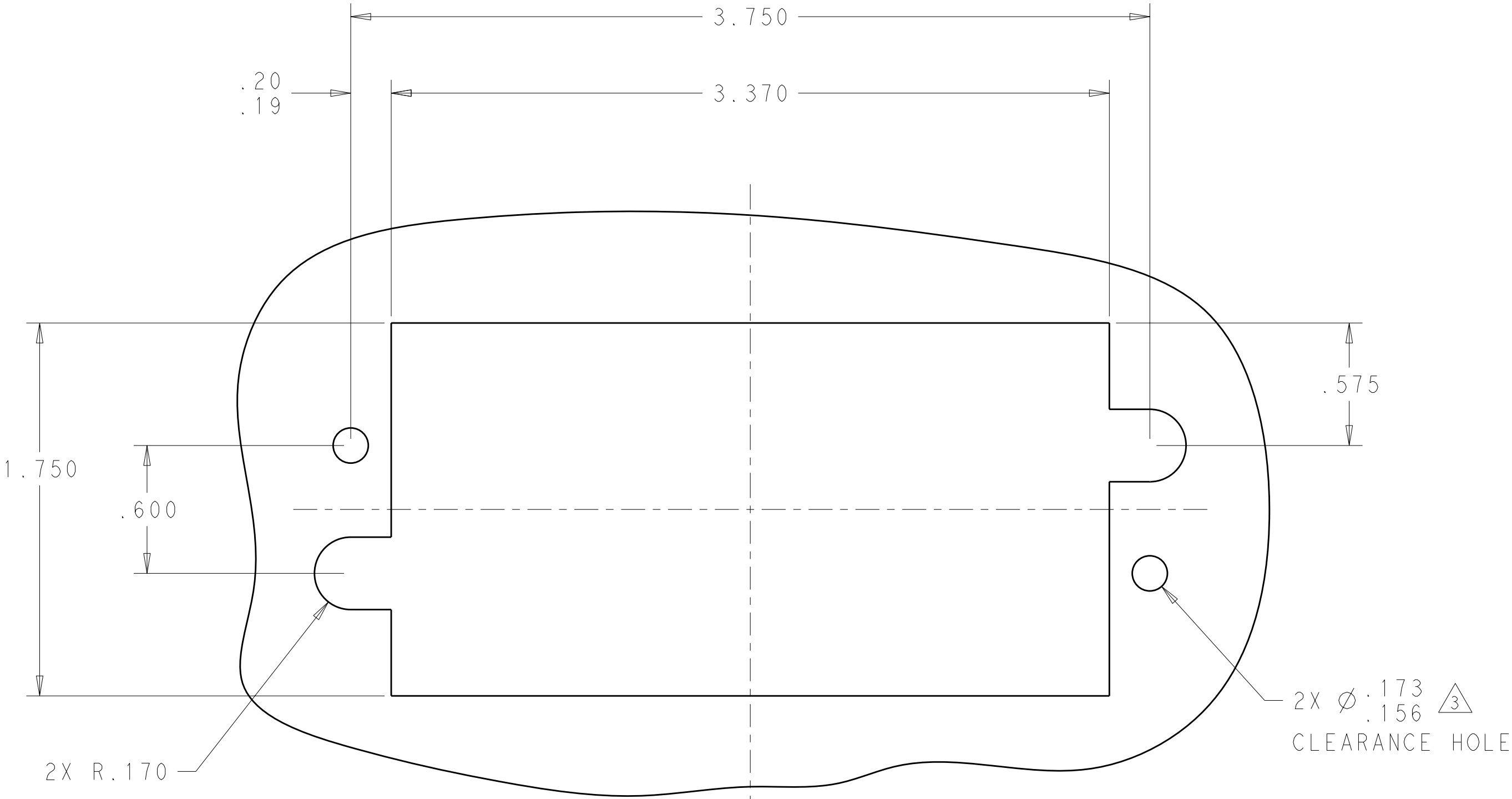
SOCKET PANEL MOUNT CUT-OUT
