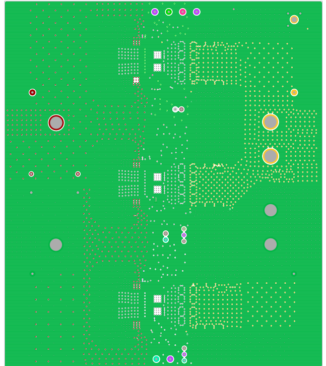
Figure 10. Layer 4
