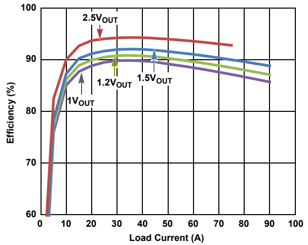
Figure 19. 5V Input
