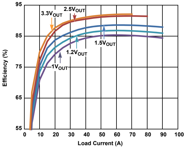
Figure 18. 12V Input
