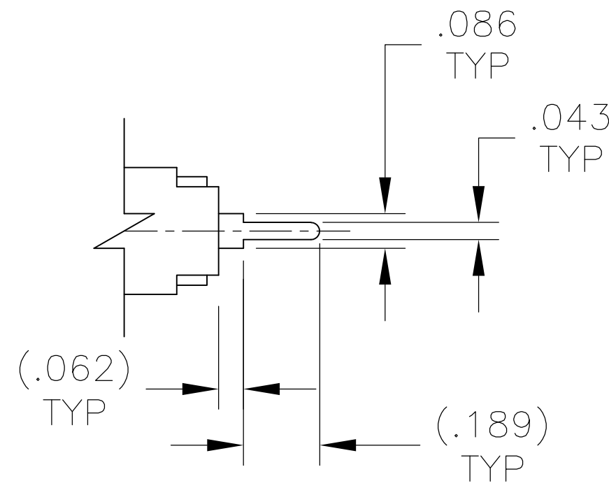
PC TERMINAL
