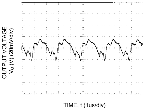
Fig-33. Typical output ripple and noise (CO=2X47uF ceramic, VIN = 12V, Io = Io,max, ).
