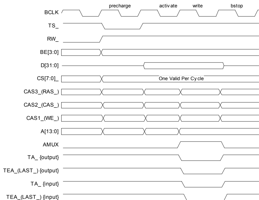
Figure 13: SDRAM normal write
