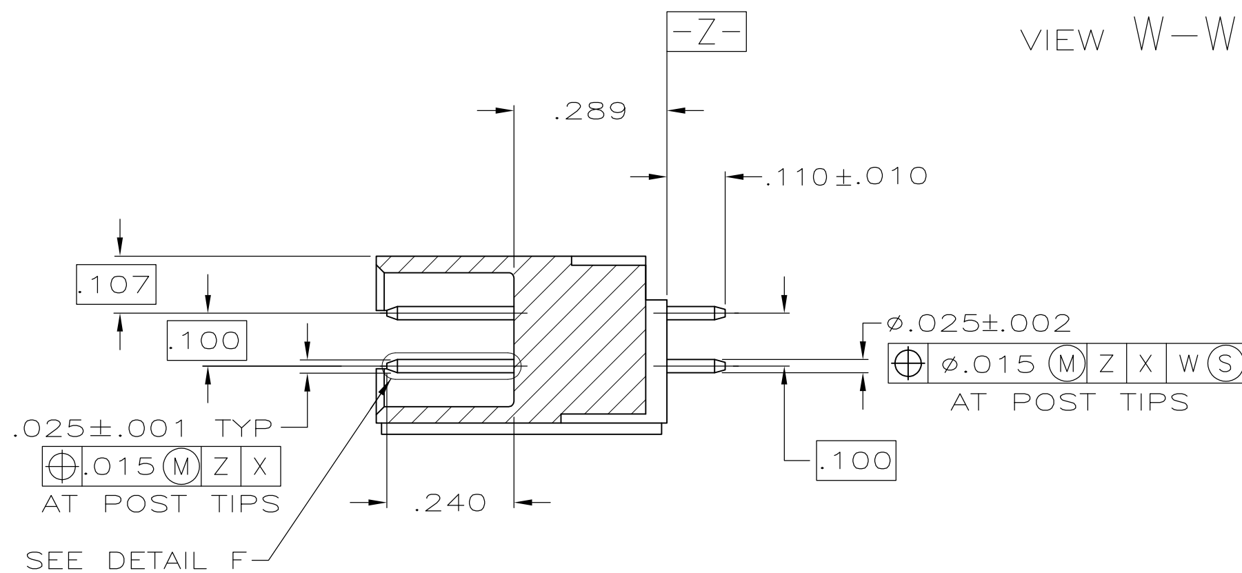
SECTION Z-Z
