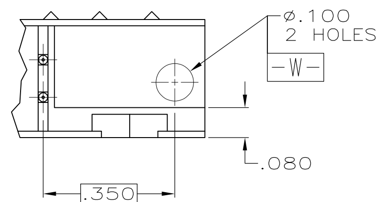
VIEW W-W
