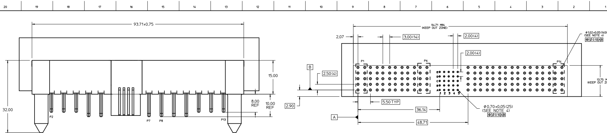
RECOMMENDED PCB LAYOUT AND KEEP-OUT ZONE
