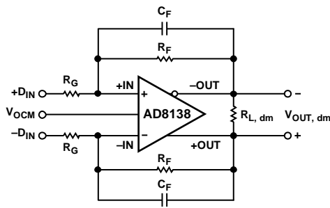
Figure 42. Circuit Definitions
