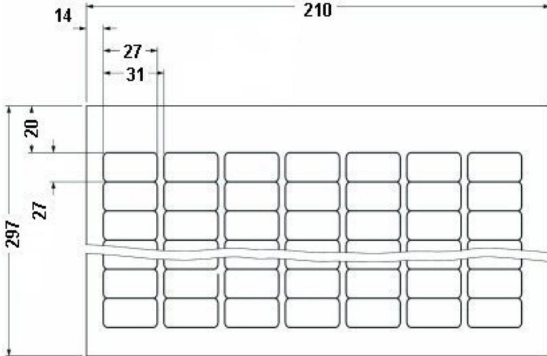
Dimensional drawing
