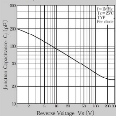
Junction Capacitance
