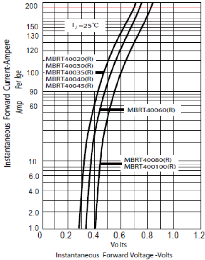
Figure.1-Typical Forward Characteristics
