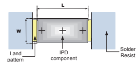
(0603 PCB footprint)
