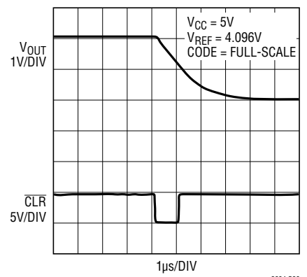
Hardware \overline{\text{CLR}} to Mid-Scale
