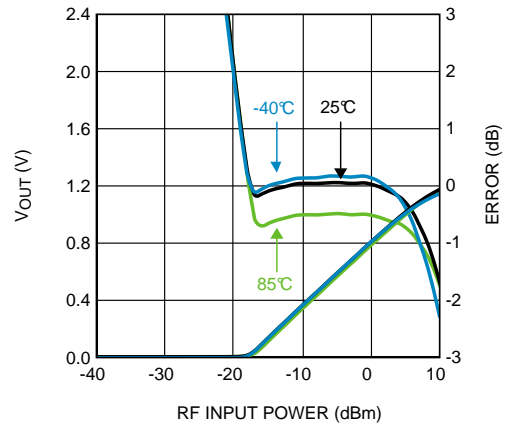
Figure 40. Output Voltage and Log Conformance Error vs. RF Input Power at 8000 MHz
