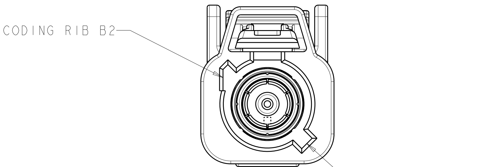
DETAIL I
