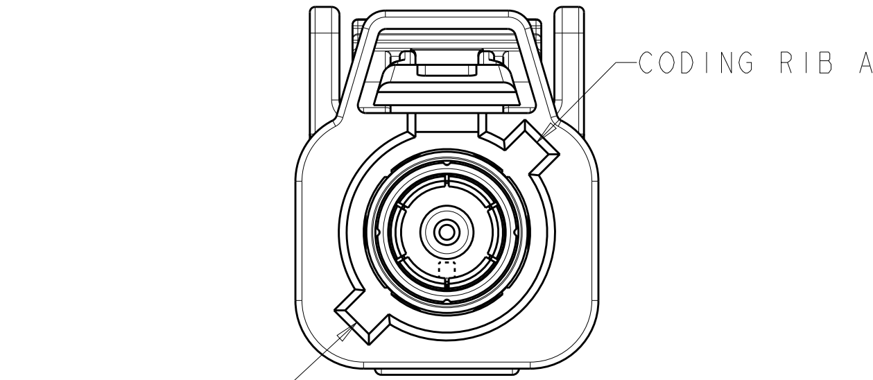
DETAIL C
