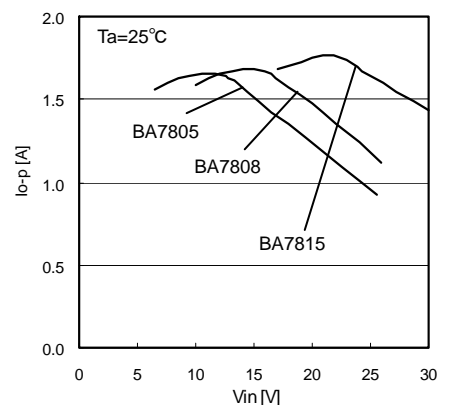
Fig.18 Peak Output Current
