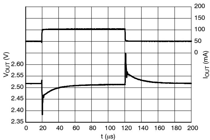
Figure 35. Load Transients, 2.5 V Version, t_R = t_F = 0.5 \mu\text{s} , V_{IN} = 3.5 \text{ V}
