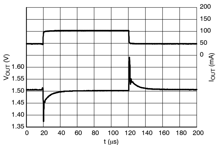
Figure 34 - Load Transients, 1.5 V Version, t_R = t_F = 0.5 \mu\text{s} , V_{IN} = 1.5 \text{ V}
