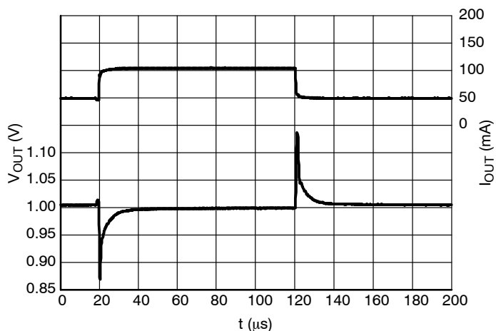
Figure 33. Load Transients, 1.0 V Version, t_R = t_F = 0.5 \mu\text{s} , V_{IN} = 2.0 \text{ V}
