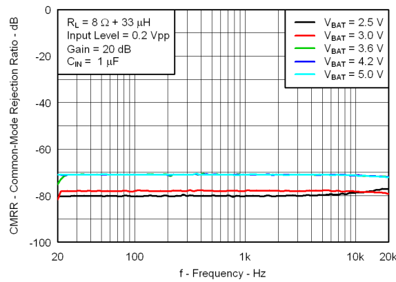
Figure 21. Common Mode Rejection Ratio vs Frequency
