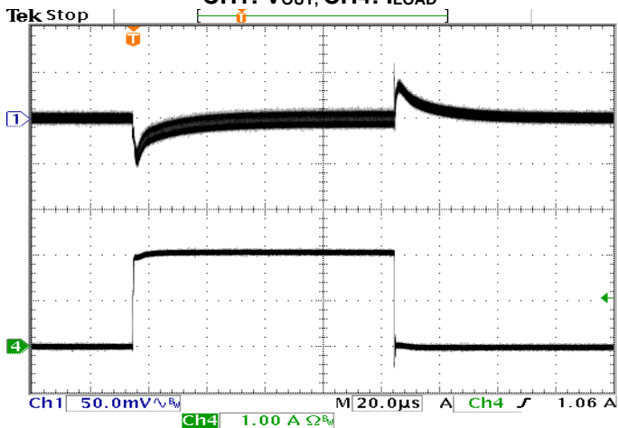
Transient Response at V_{IN} = 5\text{ V} V_{OUT} = 1.2\text{ V} , C_{OUT} = 1 \times 47\ \mu\text{F} (0-2 A Load Step, slew rate \geq 10\text{ A}/\mu\text{s} ) CH1: V_{OUT} , CH4: I_{LOAD}
