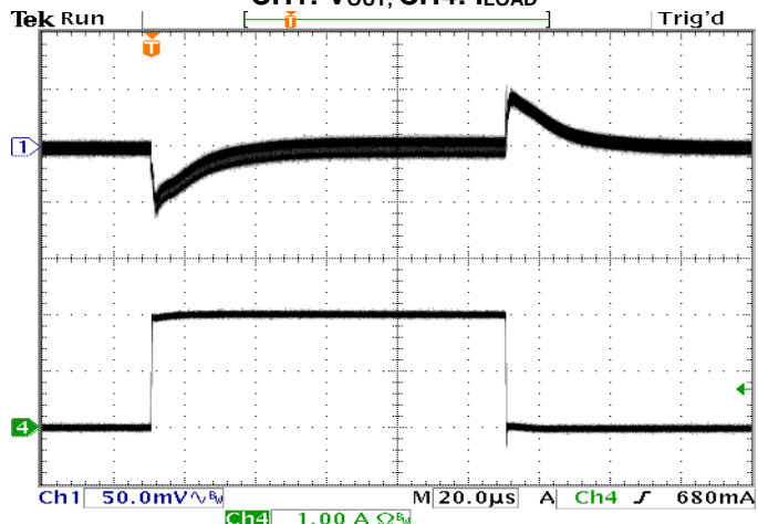
Transient Response at V_{IN} = 5\text{ V} V_{OUT} = 3.3\text{ V} , C_{OUT} = 1 \times 47\ \mu\text{F} (0-2 A Load Step, slew rate \geq 10\text{ A}/\mu\text{s} ) CH1: V_{OUT} , CH4: I_{LOAD}
