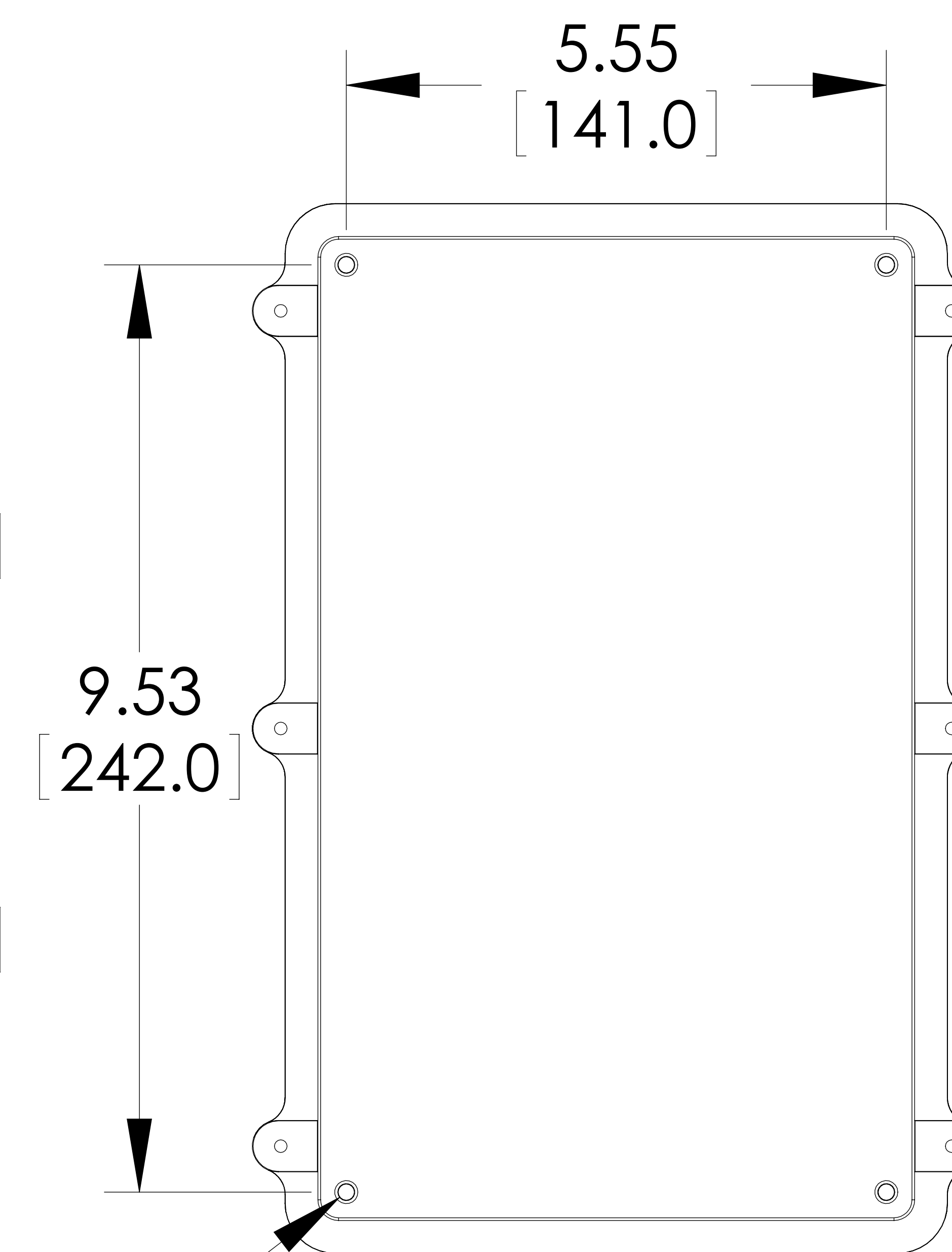
BOTTOM VIEW
