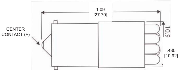
Measurements are typical Dimensions are inches [mm]
