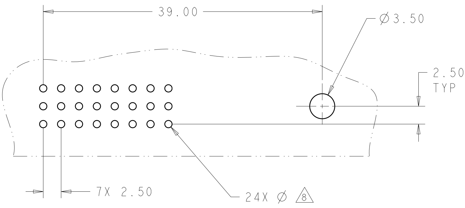
PRINTED CIRCUIT LAYOUT COMPONENT SIDE
