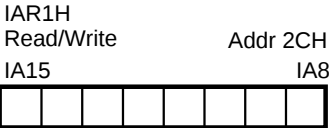
Figure 38. DMA I/O Address Registers
