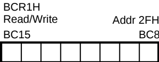
Figure 39. DMA 1 Byte Count Registers
