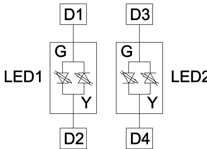
LED CONFIGURATION FOR 6605706-6 AND 5-6605706-6
