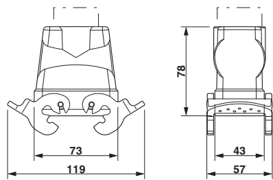
Dimensional drawing
