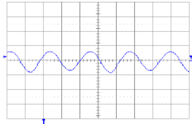
Fig. 2.5V.13: Input reflected-ripple current, c (100 mA/div.), measured at input terminals at full rated load current and V_{in} = 48\ \text{V} . Refer to Fig. 2.5V.12 for test setup. Time scale: 1\ \mu\text{s}/\text{div.}
