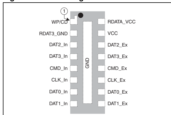
Figure 1. Pin configuration
