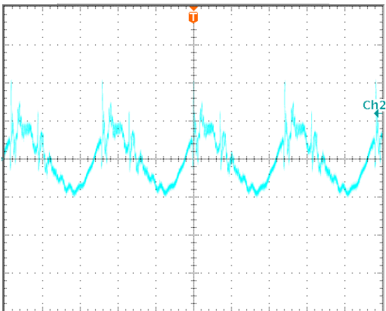
Output voltage ripple at nominal input voltage and max load current (20 mV/div, 2us/div) Load cap: 10µF, tantalum capacitor and 1µF ceramic capacitor. Bandwidth: 20 MHz.
