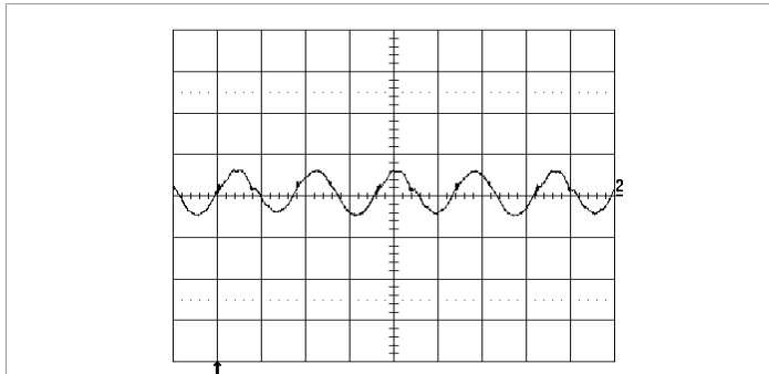
Output voltage ripple at: T_{P1}, T_{P3} = +25^{\circ}\text{C} , V_1 = 53\text{ V} , I_O = 35\text{ A} resistive load. Trace: output voltage (50 mV/div.). Time scale: (2 μs/div.).
