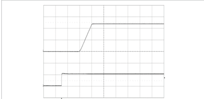
Start-up enabled by connecting V_1 at: T_{P1}, T_{P3} = +25^{\circ}\text{C} , V_1 = 53\text{ V} , I_O = 35\text{ A} resistive load. Top trace: output voltage (5 V/div.). Bottom trace: input voltage (50 V/div.). Time scale: (10 ms/div.).
