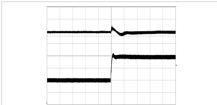
Output voltage response to input voltage transient at: T_{P1}, T_{P3} = +25^{\circ}\text{C} , V_1 = 36-75\text{ V} , I_O = 17\text{ A} resistive load, C_O = 3.5\text{ mF} . Top trace: output voltage (2 V/div.). Bottom trace: input voltage (20 V/div.). Time scale: (0.5 ms/div.).
