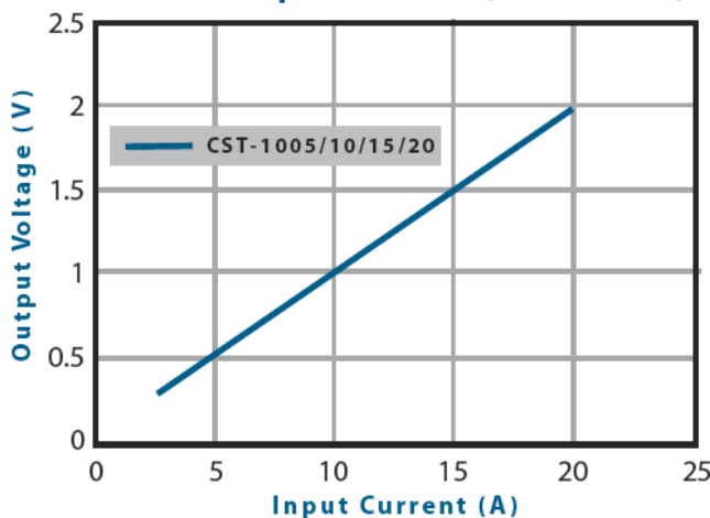
Vout vs Input current (100Ω load)
